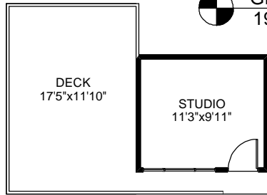
STUDIO 130 SQ.FT
