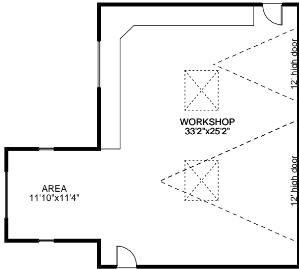
WORKSHOP 1029 SQ.FT
